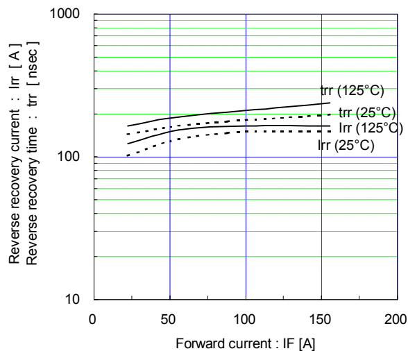
Reverse recovery characteristics (typ.) V_{CC}=900V , V_{GE}=\pm 15V , R_g=4.7\Omega
